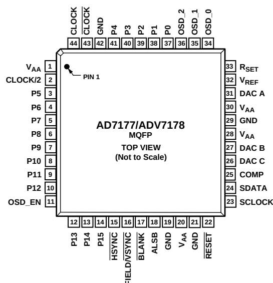
Figure 6. Pin Configuration
