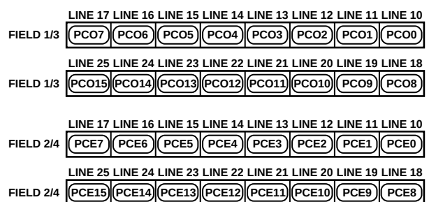
Figure 40. Pedestal Control Registers
