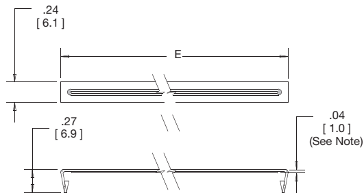
Strain Relief
