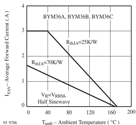
Figure 2. Max. Average Forward Current vs. Ambient Temperature
