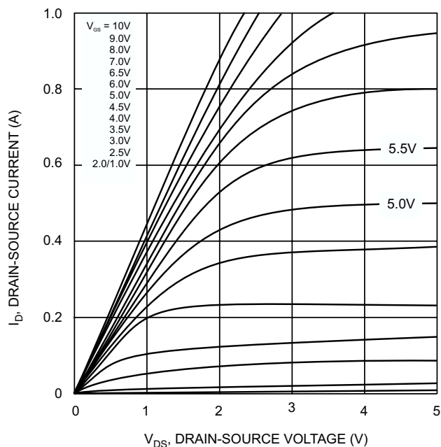
Fig. 3 On-Region Characteristics (2N7002)
