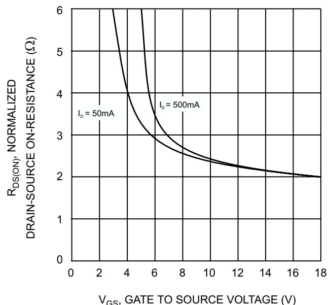
Fig. 6 On-Resistance vs. Gate-Source Voltage (2N7002)
