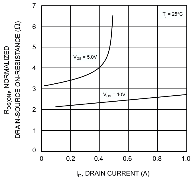
Fig. 4 On-Resistance vs Drain Current (2N7002)
