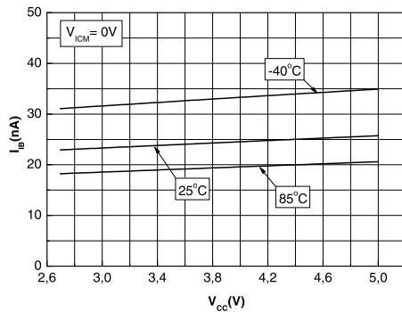
Figure 6. Input bias current versus supply voltage
