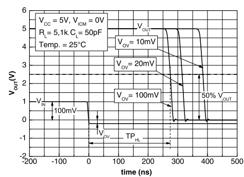
Figure 7. Response time versus overdrive with negative transition, V_{CC} = 5 V
