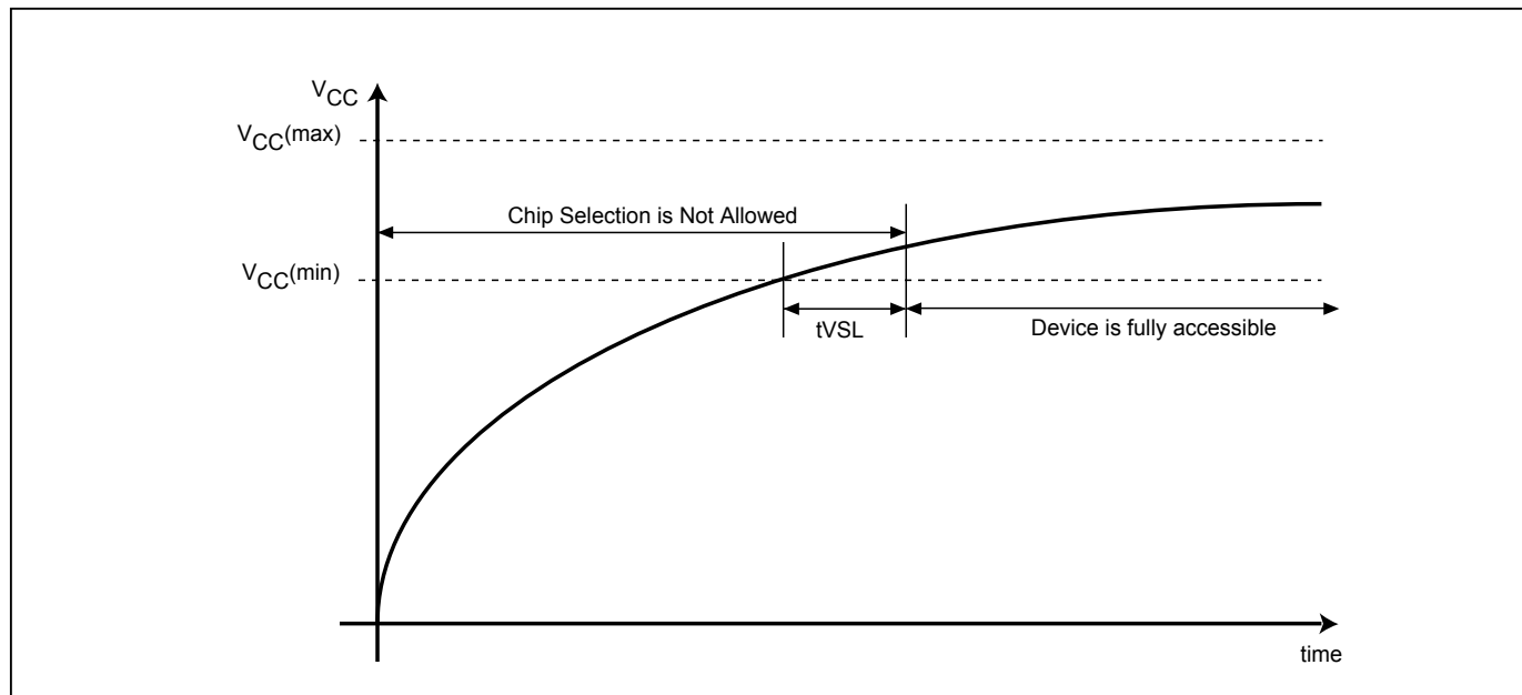
Figure 30. Power-up Timing
