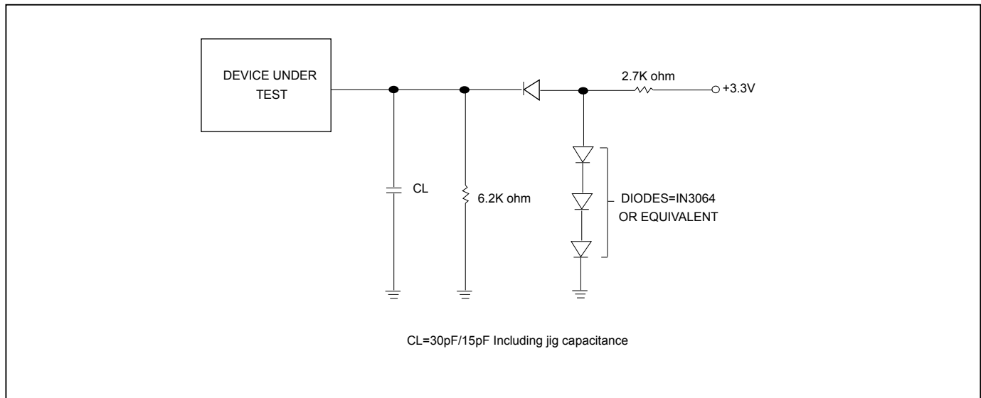
Figure 6. OUTPUT LOADING
