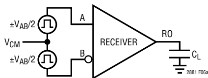
Figure 6. Receiver Propagation Delay Measurements
