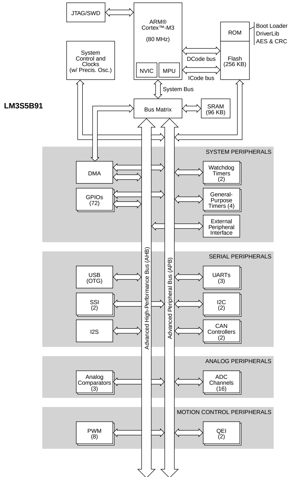
Figure 1-1. Stellaris LM3S5B91 Microcontroller High-Level Block Diagram
