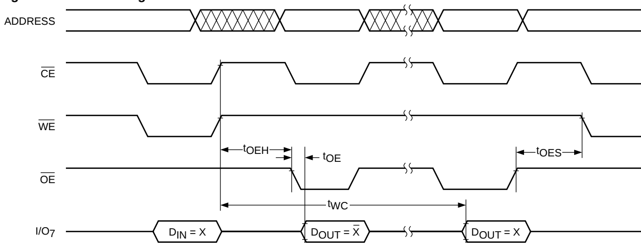
Figure 7. DATA Polling
