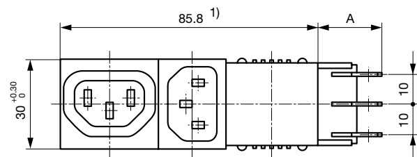
Variants 5421.X05X.XXX Mounting hole: 85.9^{+0.2}_{-0} \times 27.6^{+0.2}_{-0} A: Quick-connect terminal 6.3x0.8 mm: 22 mm A: Solder terminal 3.5x0.8 mm: 17.5 mm
