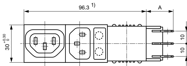
Variants 5423.XX5X.XXX Mounting hole: 96.4^{+0.2}_{-0} \times 27.6^{+0.2}_{-0} A: Quick-connect terminal 6.3x0.8 mm: 22 mm A: Solder terminal 3.5x0.8 mm: 17.5 mm
