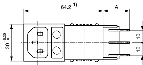
Variants 5411.XX5X.XXX Mounting hole: 63^{+0.2}_{-0} \times 27.6^{+0.2}_{-0} A: Quick-connect terminal 6.3x0.8 mm: 22 mm A: Solder terminal 3.5x0.8 mm: 17.5 mm
