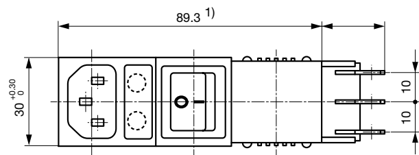
Variants 5424.XX5X.XXX Mounting hole: 87.9^{+0.2}_{-0} \times 27.6^{+0.2}_{-0} A: Quick-connect terminal 6.3x0.8 mm: 22 mm A: Solder terminal 3.5x0.8 mm: 17.5 mm
