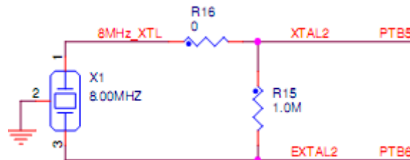
Figure 4. Main Oscillator Input
