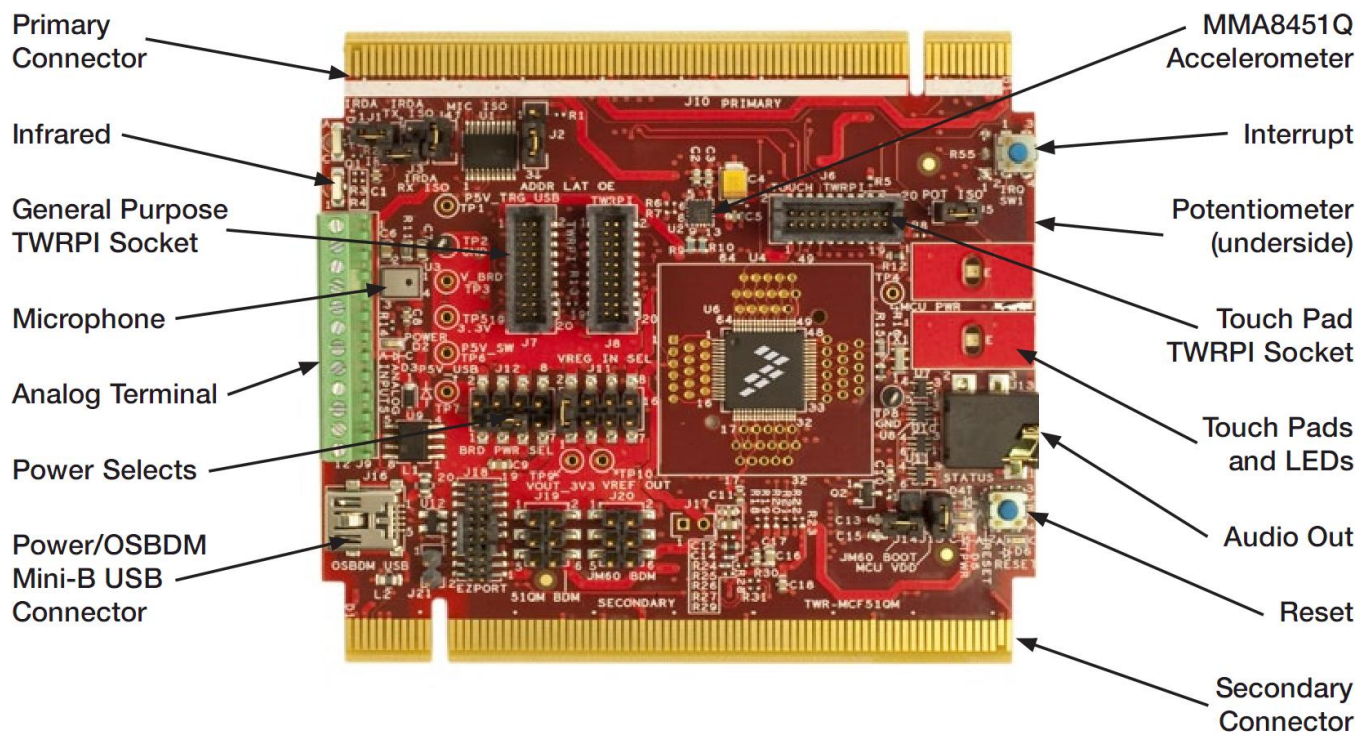
Figure 2. Callouts on front side of the TWR-MCF51QM
