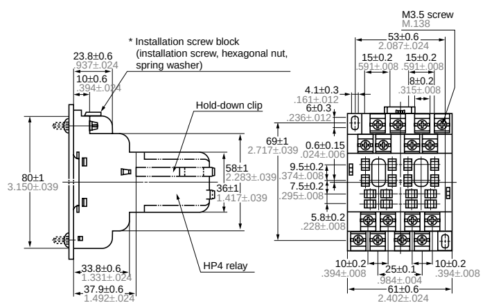
External dimensions
