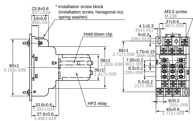
External dimensions
