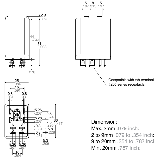
External dimensions
