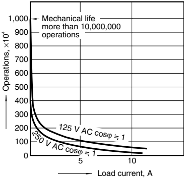
1. Life curve
