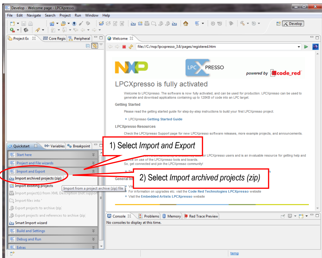
Figure 18 – LPCXpresso IDE Import Archived Project
