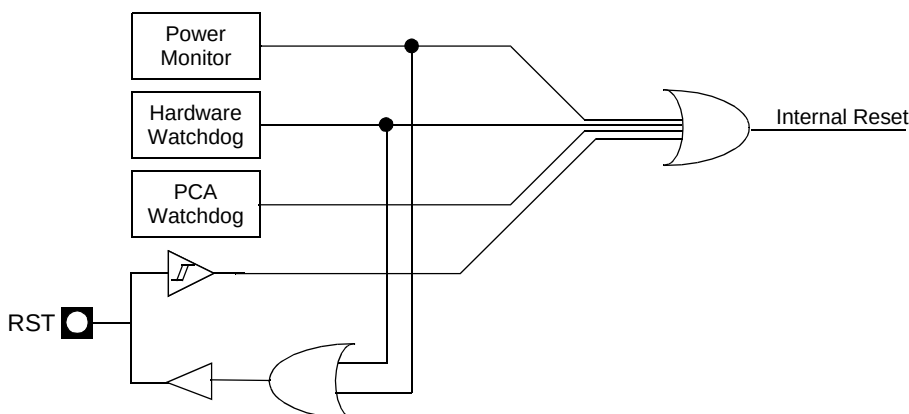
Figure 68. Reset schematic
