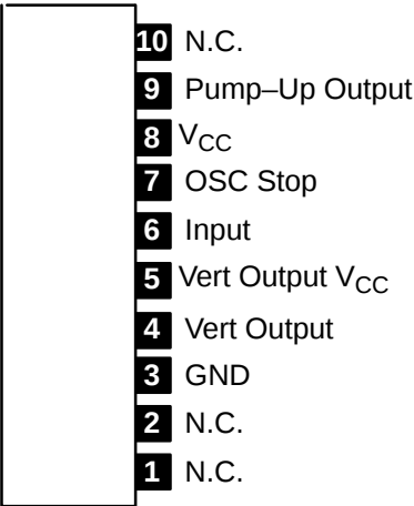
Pin Connection Diagram (Front View)
