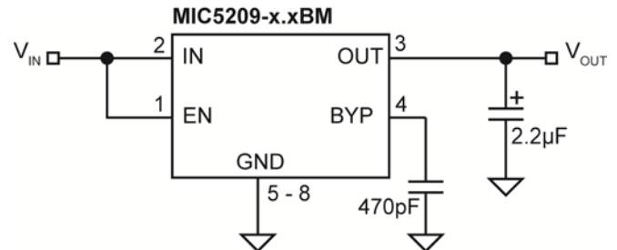
Figure 2. Ultra-Low-Noise Fixed Voltage Regulator
