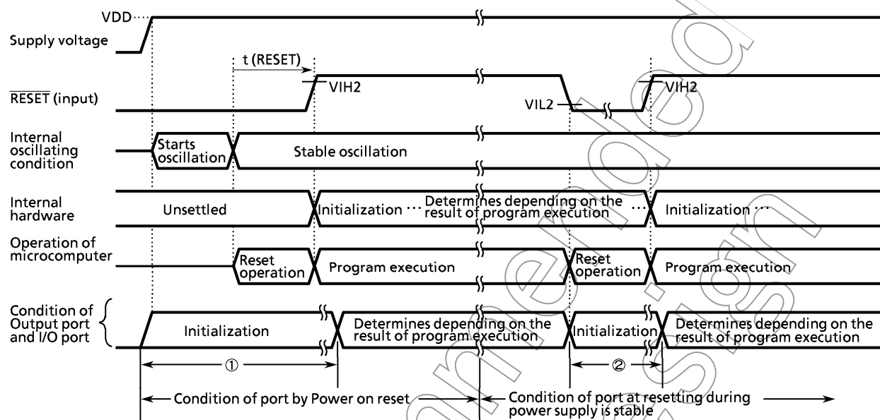
Figure 3-25. Port condition by Reset operation
