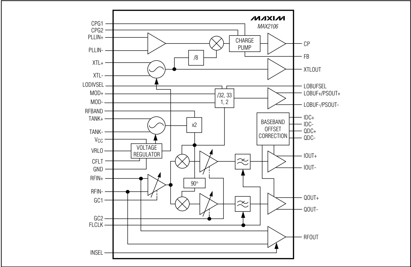
Functional Diagram
