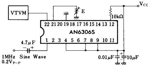
Test Circuit 4 ( G_{V1-22} )
