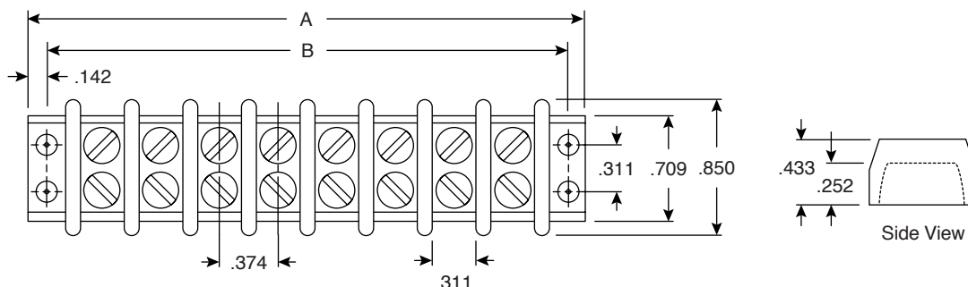
Dimensions (In.)
