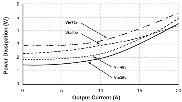
Power Dissipation vs. Output Current for 1.5V/20A PKM4318PIOA
