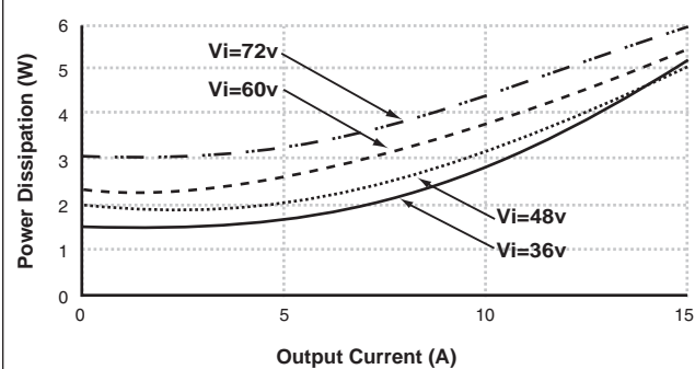
Power Dissipation vs. Output Current for 3.3V/15A PKM4510PI
