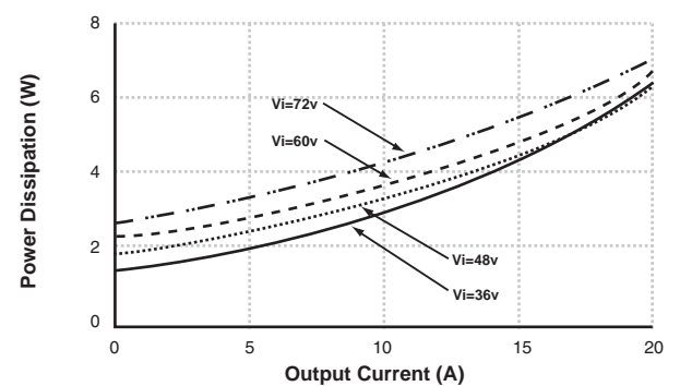
Power Dissipation vs. Output Current for 2.5V/20A PKM4519PI
