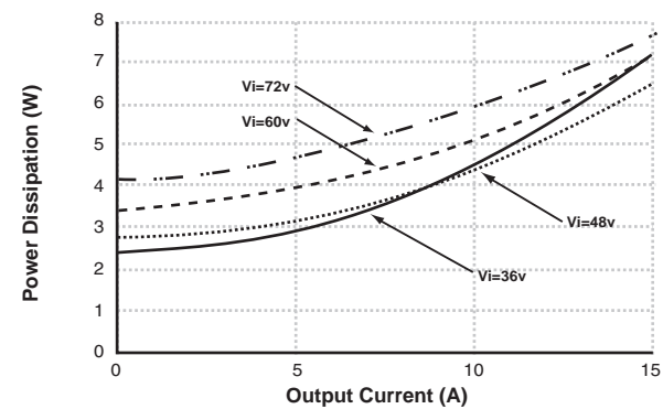
Power Dissipation vs. Output Current for 5V/15A PKM4711PI
