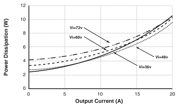
Power Dissipation vs. Output Current for 5V/20A PKM4111PI
