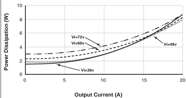
Power Dissipation vs. Output Current for 3.3V/20A PKM4610PI
