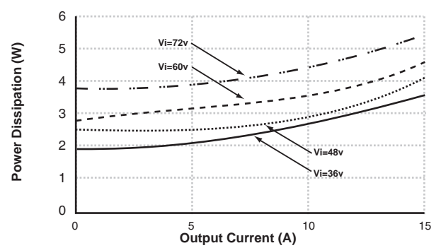
Power Dissipation vs. Output Current for 1.8V/15A PKM4218PI
