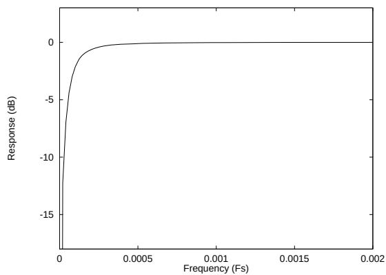
Figure 50 ADC Highpass Filter Response
