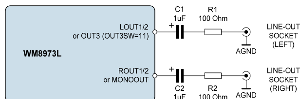
Figure 15 Recommended Circuit for Line Output
