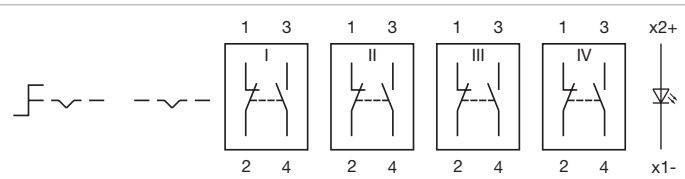
Wiring diagram 280
