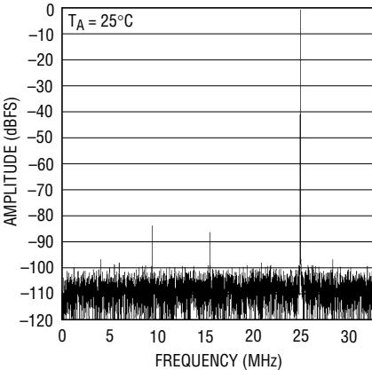
8192 Point FFT, Input Frequency = 50MHz, -1dB, 3.2V Range
