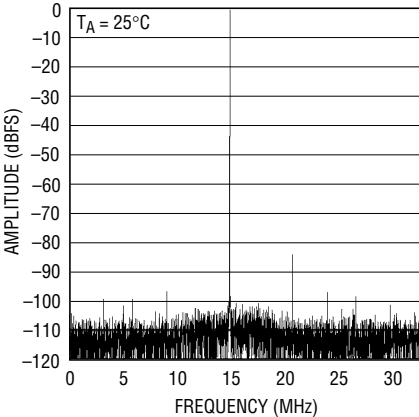
8192 Point FFT, Input Frequency = 70MHz, -1dB, 3.2V Range
