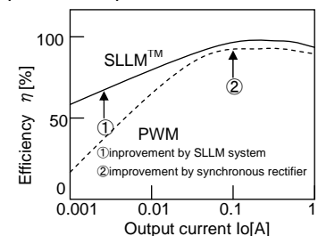
Fig.27 Efficiency
