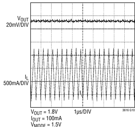
Forced Continuous Mode Operation
