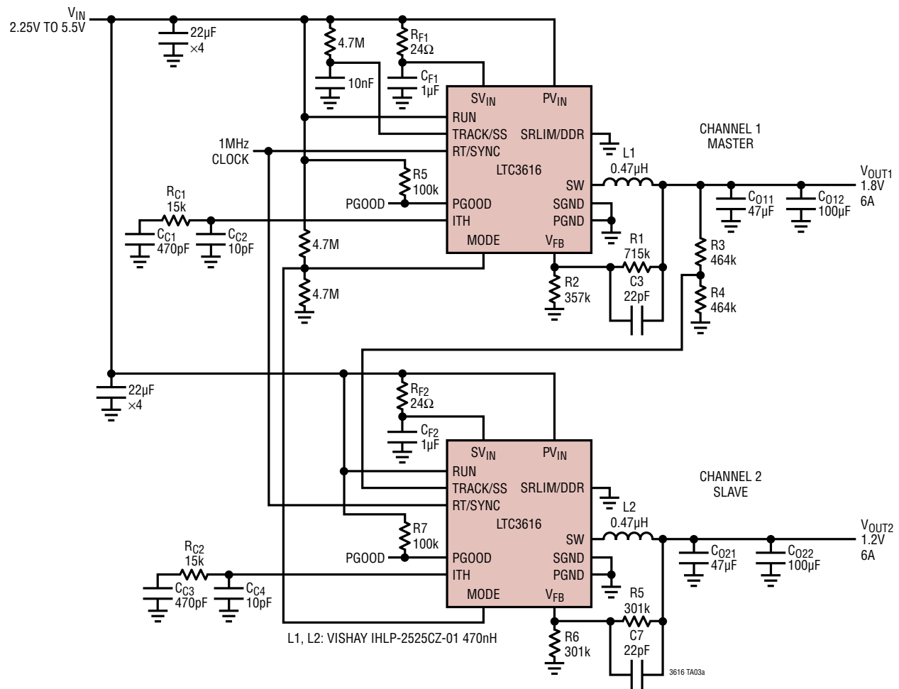
Coincident Start-Up
