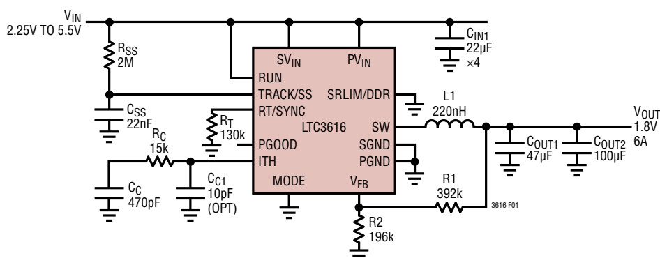
Figure 1. 1.8V, 6A Step-Down Regulator
