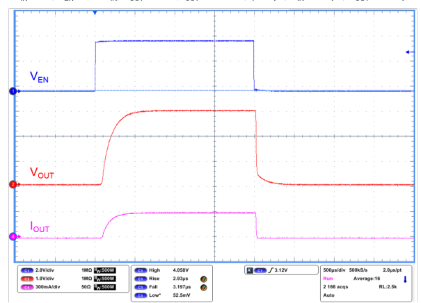
Figure 25. Enable transient
