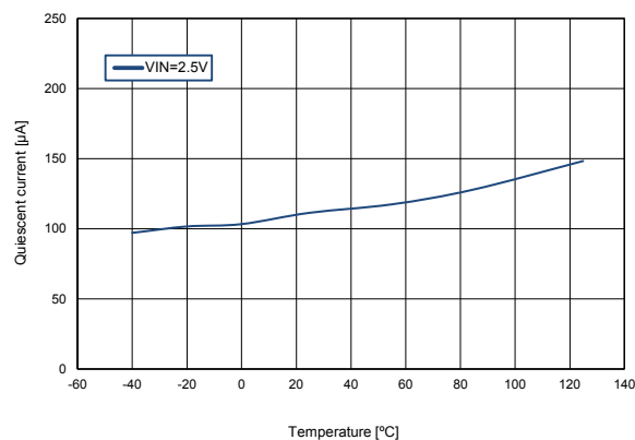
Figure 15. Quiescent current vs. temperature (I_{OUT} = 300 \text{ mA})
