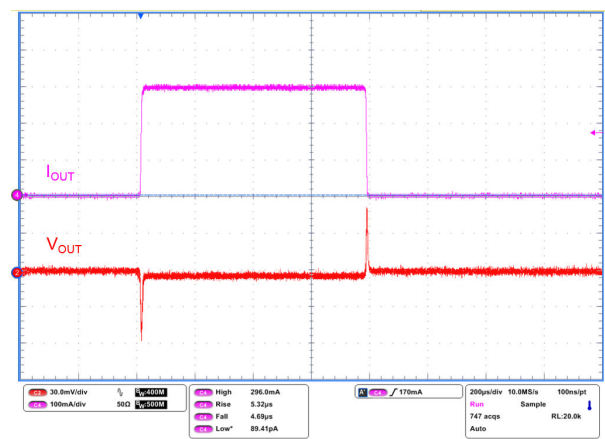
Figure 25. Enable transient
