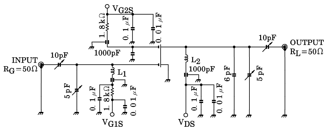
Fig.1 200MHz, G_{ps} , NF TEST CIRCUIT
