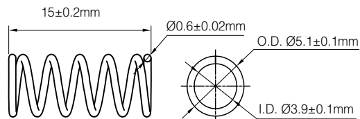
COMPRESSION SPRING:
