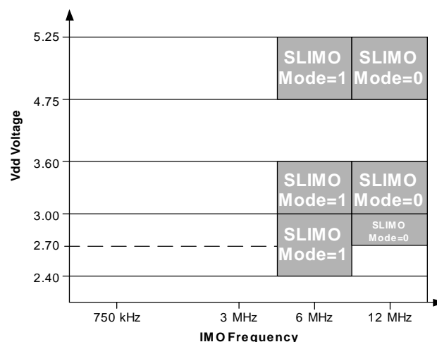
Figure 2-1b. IMO Frequency Trim Options
