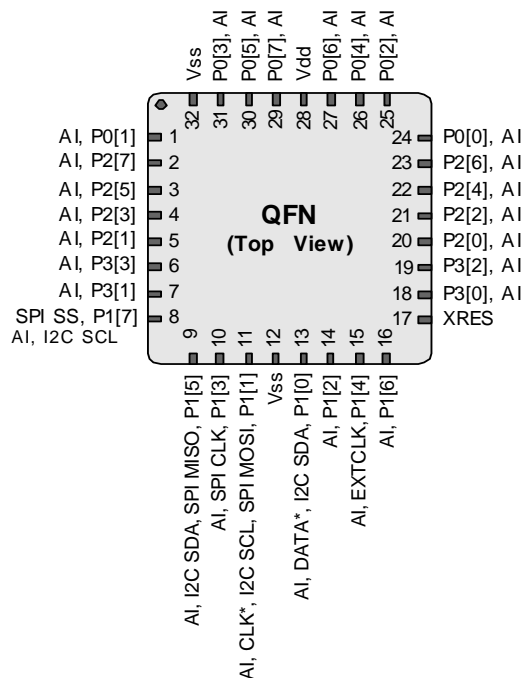
CY8C20434 32-Pin PSoC Device
