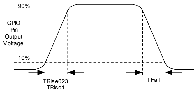
Figure 2-2. GPIO Timing Diagram
