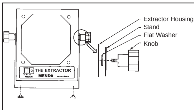
Figure 2: Installing stand assembly
