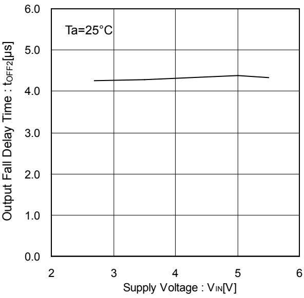
Figure 23. Output Fall Delay Time vs Supply Voltage
