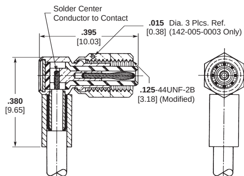
Right-Angle Plug 1
