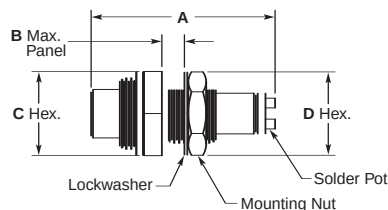
Fig. 2 Slide-On Series or Screw-On Series
