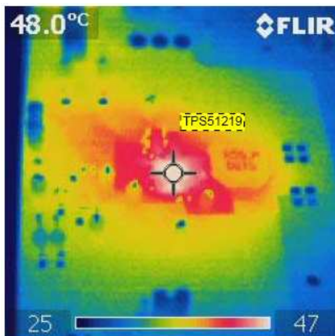
Figure 82. TPS51219 Thermal
