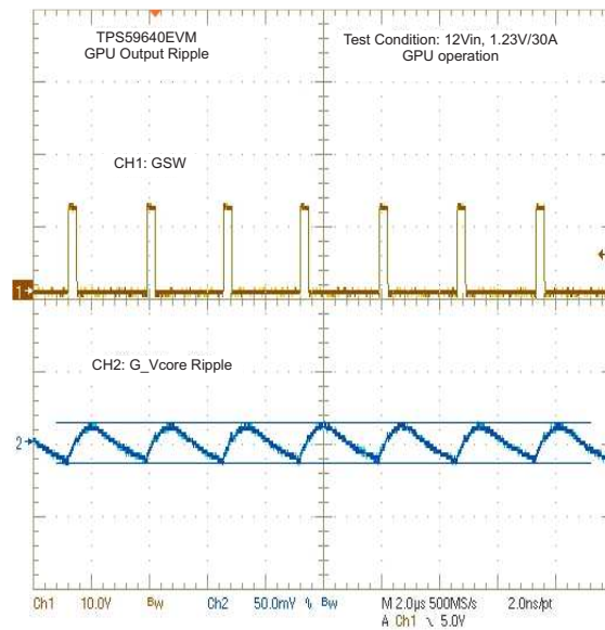
Figure 65. GPU Switching Node and Ripple
