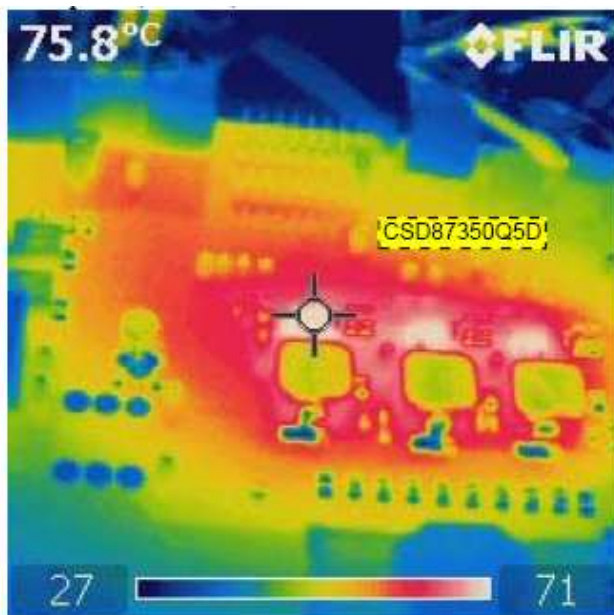
Figure 31. CPU3 MOSFET
