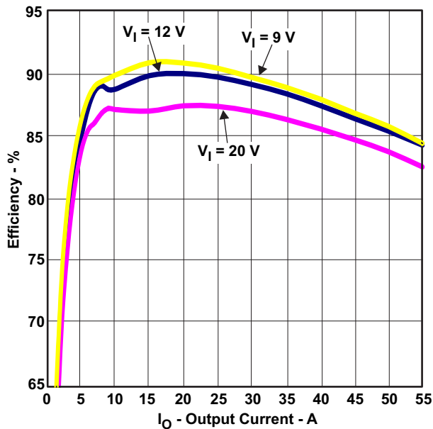
Figure 33. CPU2 Efficiency
