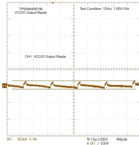
Figure 79. 1.05-V Ripple
