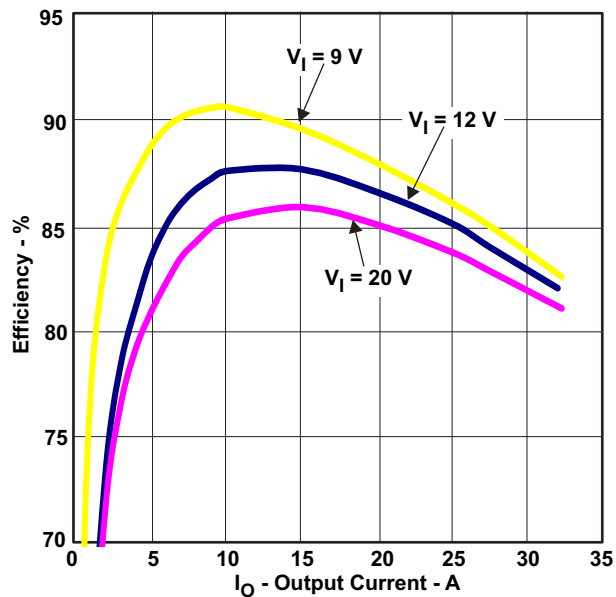
Figure 46. CPU1 Efficiency
