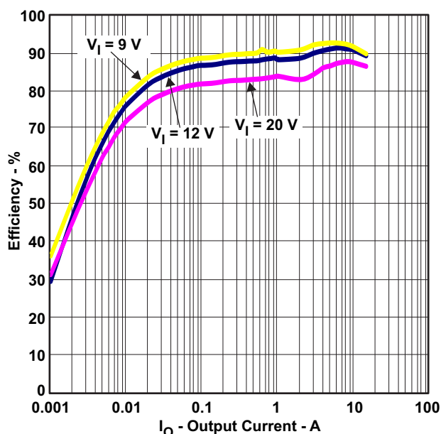
Figure 74. 1.05-V Efficiency
