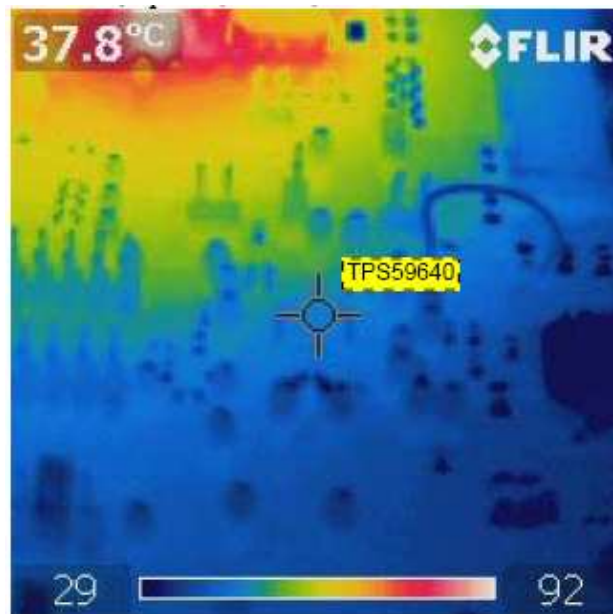
Figure 73. GPU IC
