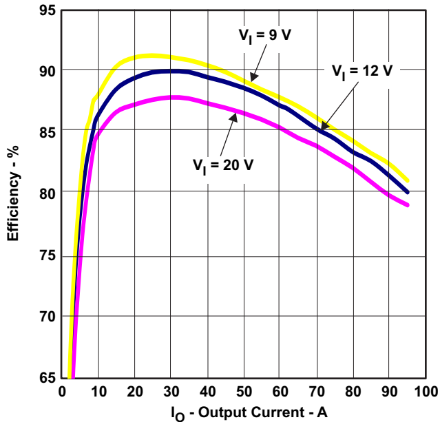
Figure 20. CPU3 Efficiency
