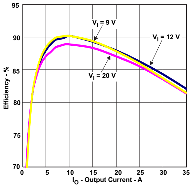
Figure 60. GPU Efficiency
