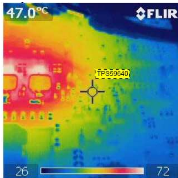
Figure 32. CPU3 IC
