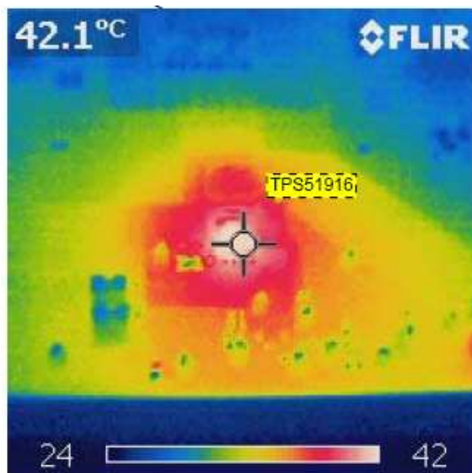
Figure 91. TPS51916 Thermal
