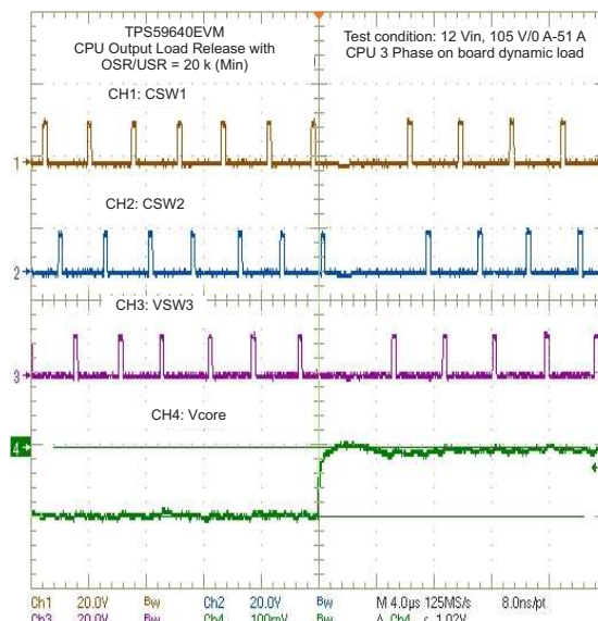
Figure 29. CPU3 Output Load Release With OSR/USR 20k (Min)
