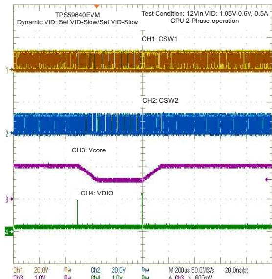
Figure 38. CPU2 Dynamic VID: SetVID-Slow/Slow
