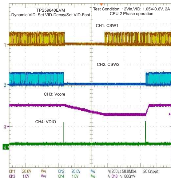
Figure 40. CPU2 Dynamic VID: SetVID-Decay/Fast
