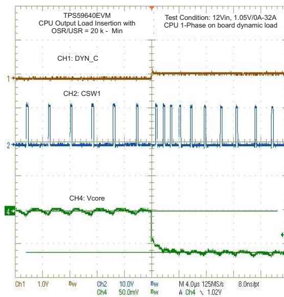
Figure 55. CPU1 Output Load Insertion With OSR/USR 20k (Min)
