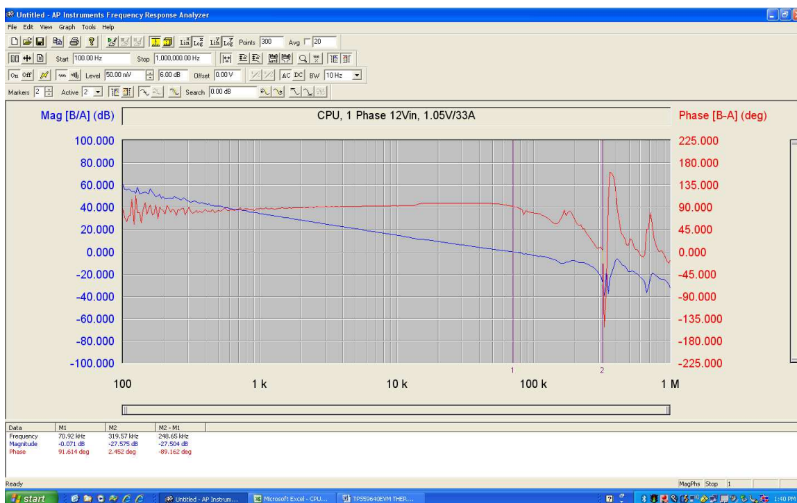
Figure 57. CPU1 Bode Plot at 12Vin, 1.05 V/33 A
