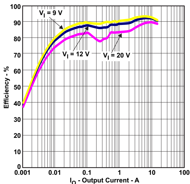
Figure 83. 1.2-V Efficiency
