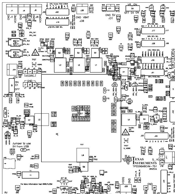
Figure 92. TPS59640EVM-751 Top Layer Assembly Drawing (Top View)
