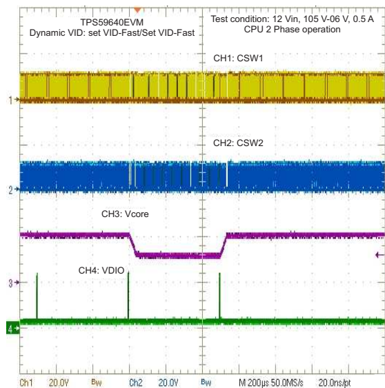
Figure 26. CPU3 Dynamic VID:SetVID-Fast/Fast
