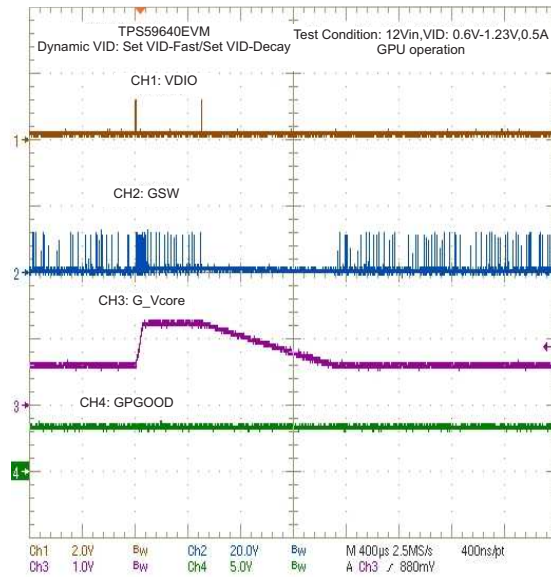
Figure 68. GPU Dynamic VID: SetVID-Fast/Set VID-Decay
