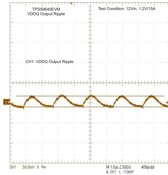
Figure 88. 1.2-V Ripple
