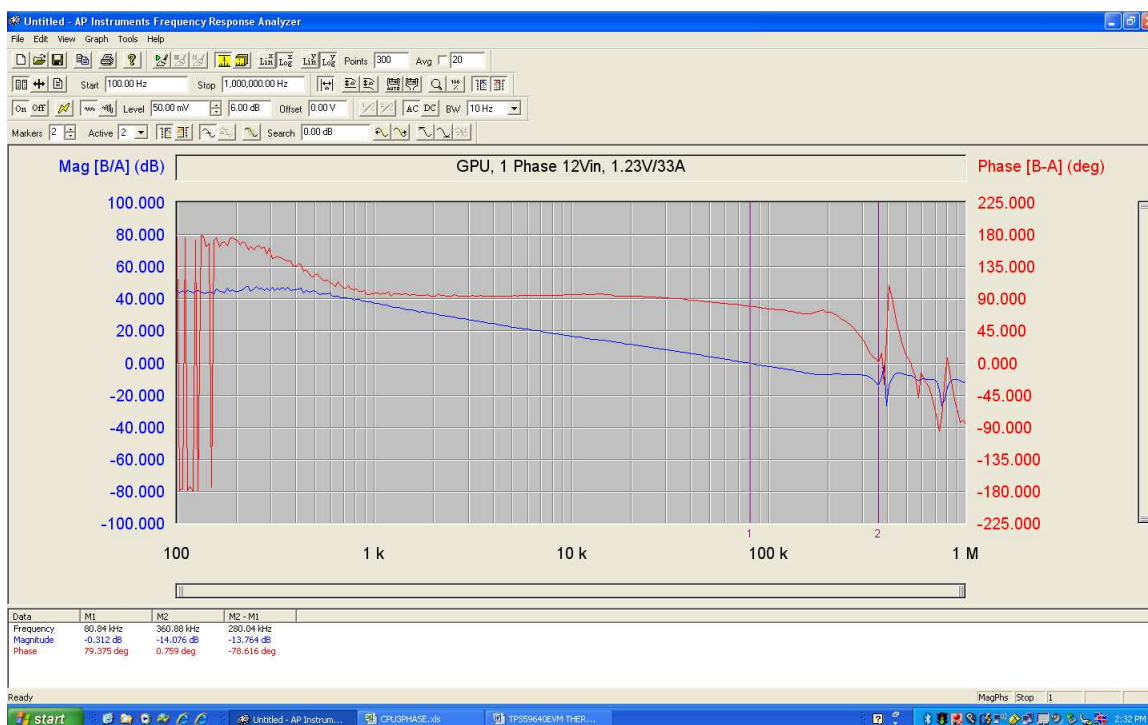
Figure 71. GPU Bode Plot at 12Vin, 1.23 V/33 A
