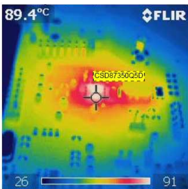
Figure 72. GPU MOSFET
