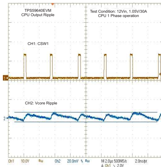
Figure 51. CPU1 Switching Node and Ripple
