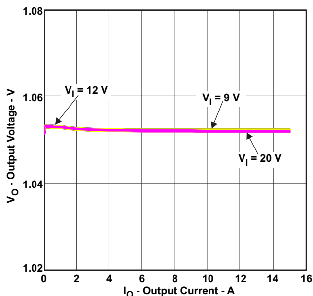
Figure 75. 1.05-V Load Regulation
