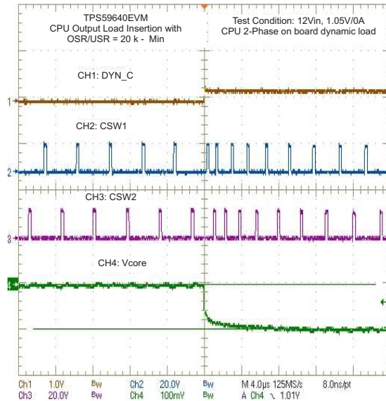
Figure 41. CPU2 Output Load Insertion With OSR/USR 20k (Min)
