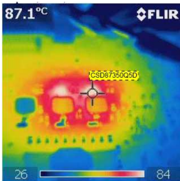
Figure 44. CPU2 MOSFET
