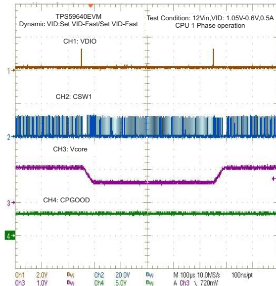
Figure 53. CPU1 Dynamic VID: SetVID-Fast/Fast
