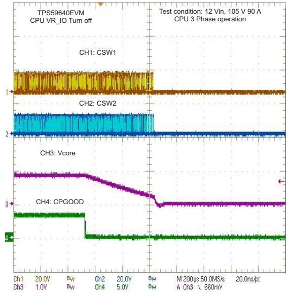
Figure 23. CPU3 Enable Turnoff
