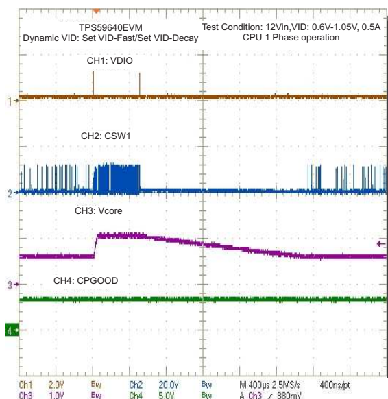
Figure 54. CPU1 Dynamic VID: SetVID-Fast/Set VID-Decay
