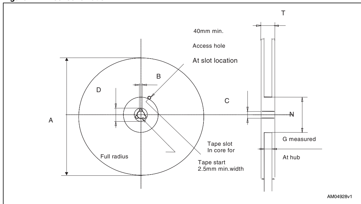
Figure 14. Reel schematic
