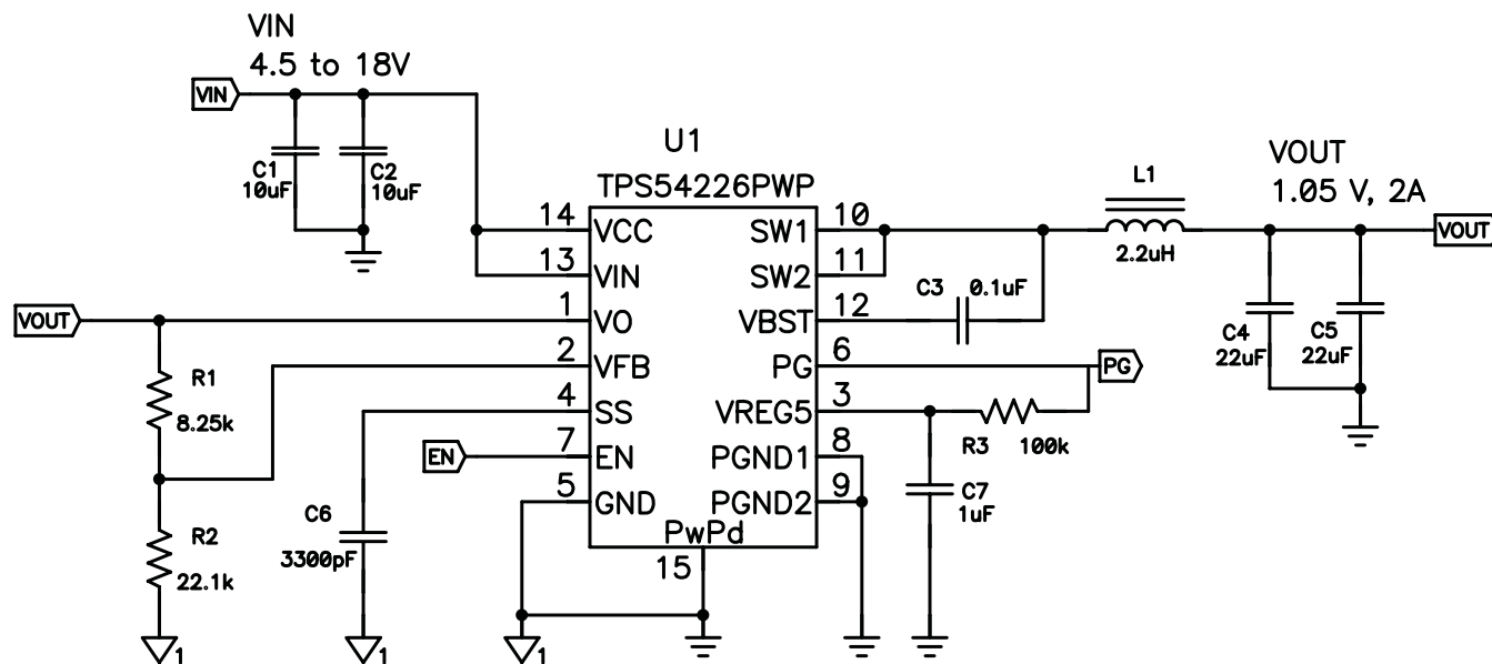
Figure 14. Schematic Diagram
