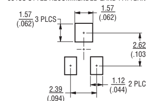
3313S STYLE RECOMMENDED LAND PATTERN
