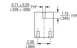
3313S STYLE RECOMMENDED LAND PATTERN
