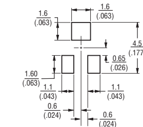
3313J STYLE RECOMMENDED LAND PATTERN
