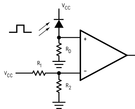
FIGURE 6. IR Receiver
