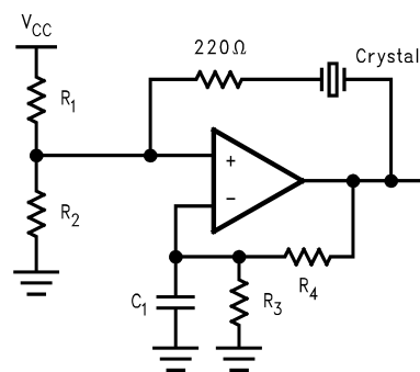
FIGURE 5. Crystal Oscillator
