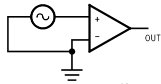
FIGURE 3. Zero-Crossing Detector
