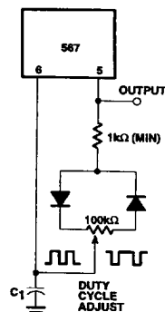
Pulse Generator
