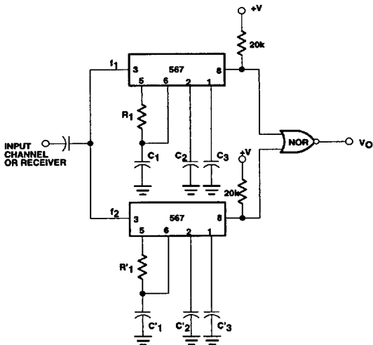
Dual-Tone Decoder
