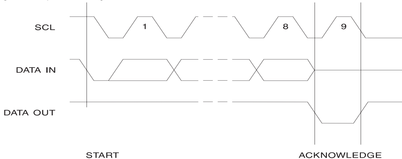
Figure 6. Output Acknowledge
