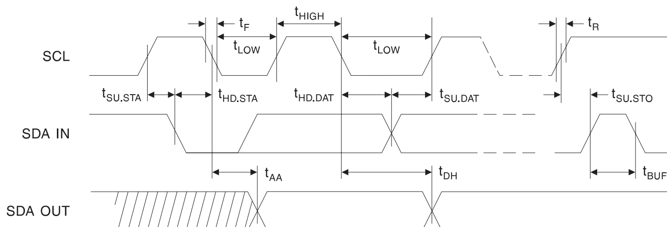
Figure 4. Bus Timing
