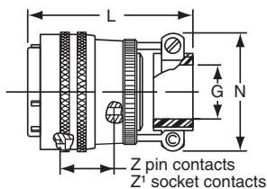
TERMINATION ASSEMBLIES “CE” (SR) Strain Relief
