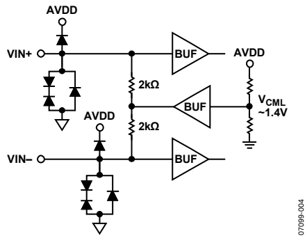
Figure 6. Analog Inputs ( V_{CML} = \sim 1.4\text{ V} )
