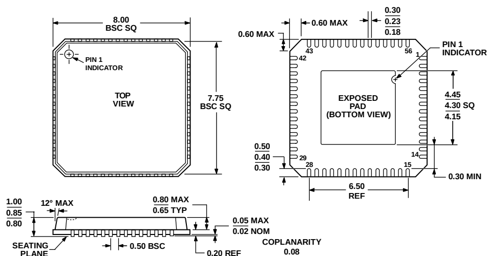
Figure 58. 56-Lead Lead Frame Chip Scale Package [LFCSP_VQ] 8 mm × 8 mm Body, Very Thin Quad (CP-56-2) Dimensions shown in millimeters
