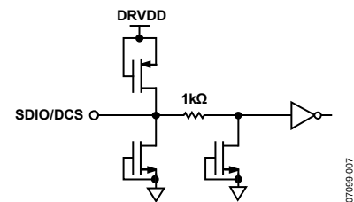
Figure 10. Equivalent SDIO/DCS Input Circuit
