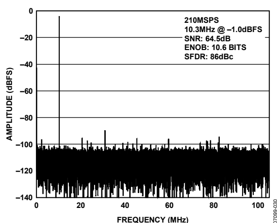
Figure 21. AD9626-210 64k Point Single-Tone FFT; 210 MSPS, 10.3 MHz
