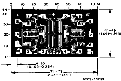
Dimensions and Pad Layout for CD4093BH
