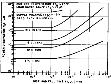
Fig. 15 - Typical power dissipation vs. rise and fall times.
