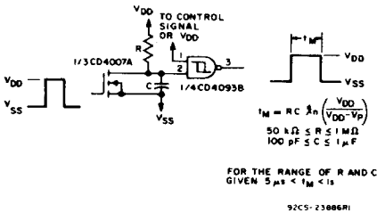
Fig. 17 - Monostable multivibrator.
