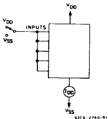
Fig. 19 - Quiescent device current test circuit.
