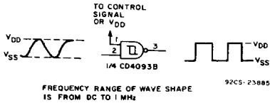
Fig. 16 - Wave shaper.
