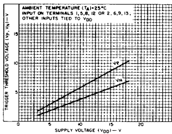
Fig. 12 — Typical trigger threshold voltage vs. V DD
