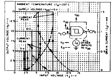
Fig. 4 - Typical current and voltage transfer characteristics.
