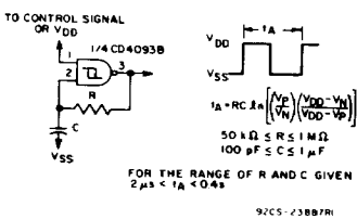
Fig. 18 - Astable multivibrator.
