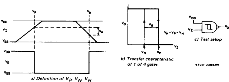
Fig. 2 — Hysteresis definition, characteristic, and test setup.
