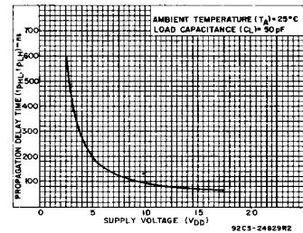
Fig. 10 — Typical propagation delay time vs. supply voltage.
