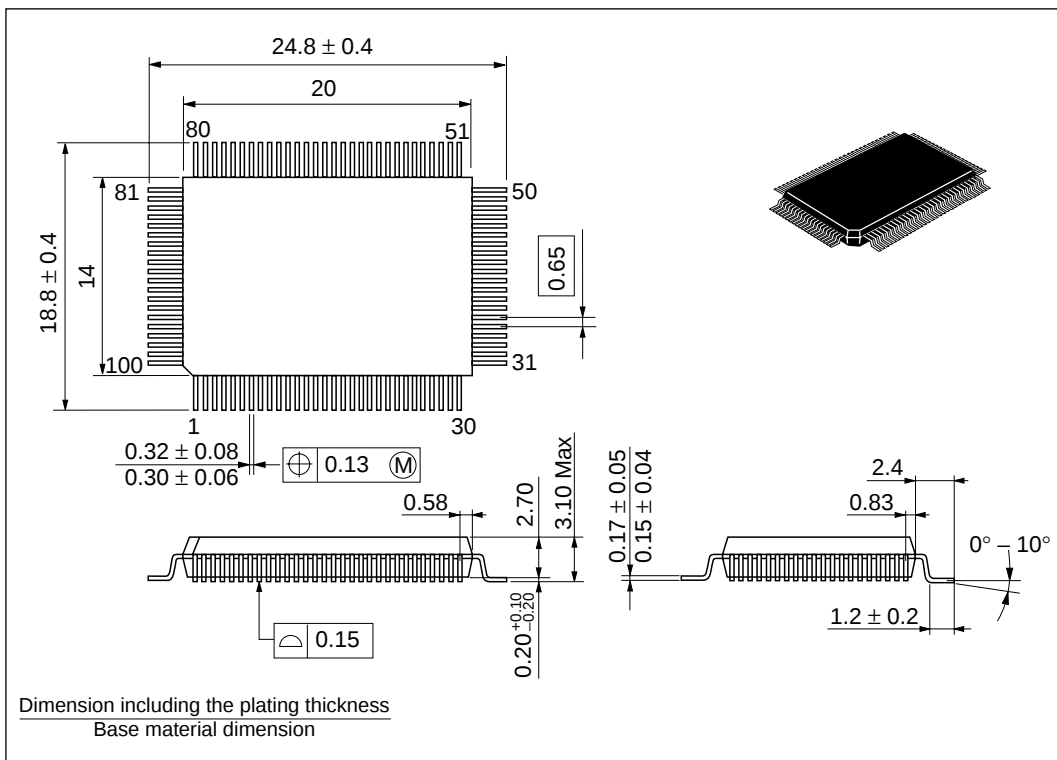
Figure F-3 Package Dimensions (FP-100A)
