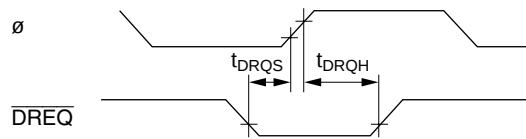
Figure 18-27 DMAC \overline{\text{DREQ}} Input Timing
