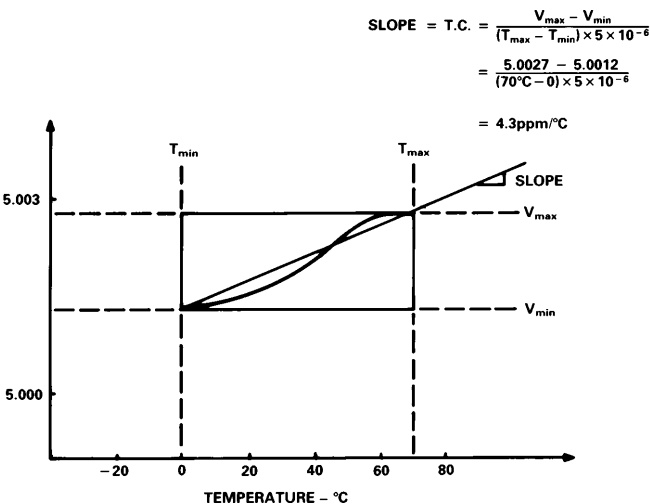
Figure 9. Typical AD586L Temperature Drift
