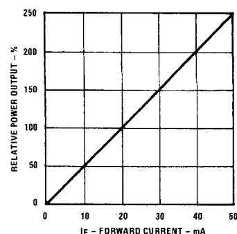
Relative Power Output vs Forward Current (LED)
