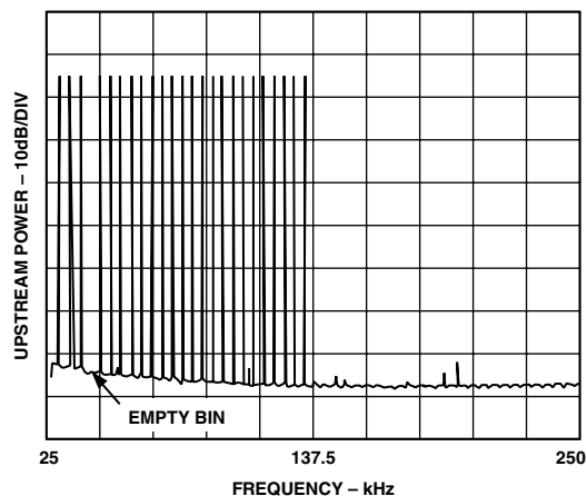
Figure 1. Upstream Transit Spectrum with Empty Bin at 45 kHz; Line Power = 12.5 dBm into 100 \Omega
