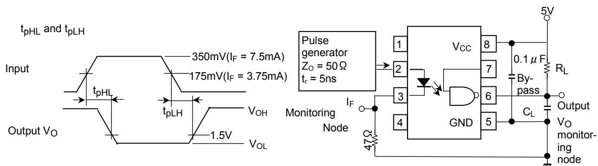
Test Circuit 1.
