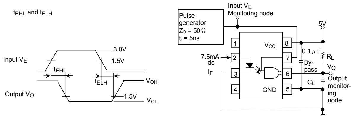
Test Circuit 2.
