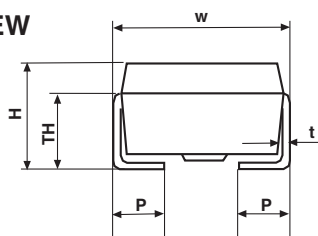
FIGURE 5 - DIMENSIONS AND IMPRINTING
