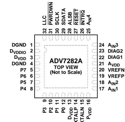
Figure 6. ADV7282A Pin Configuration
